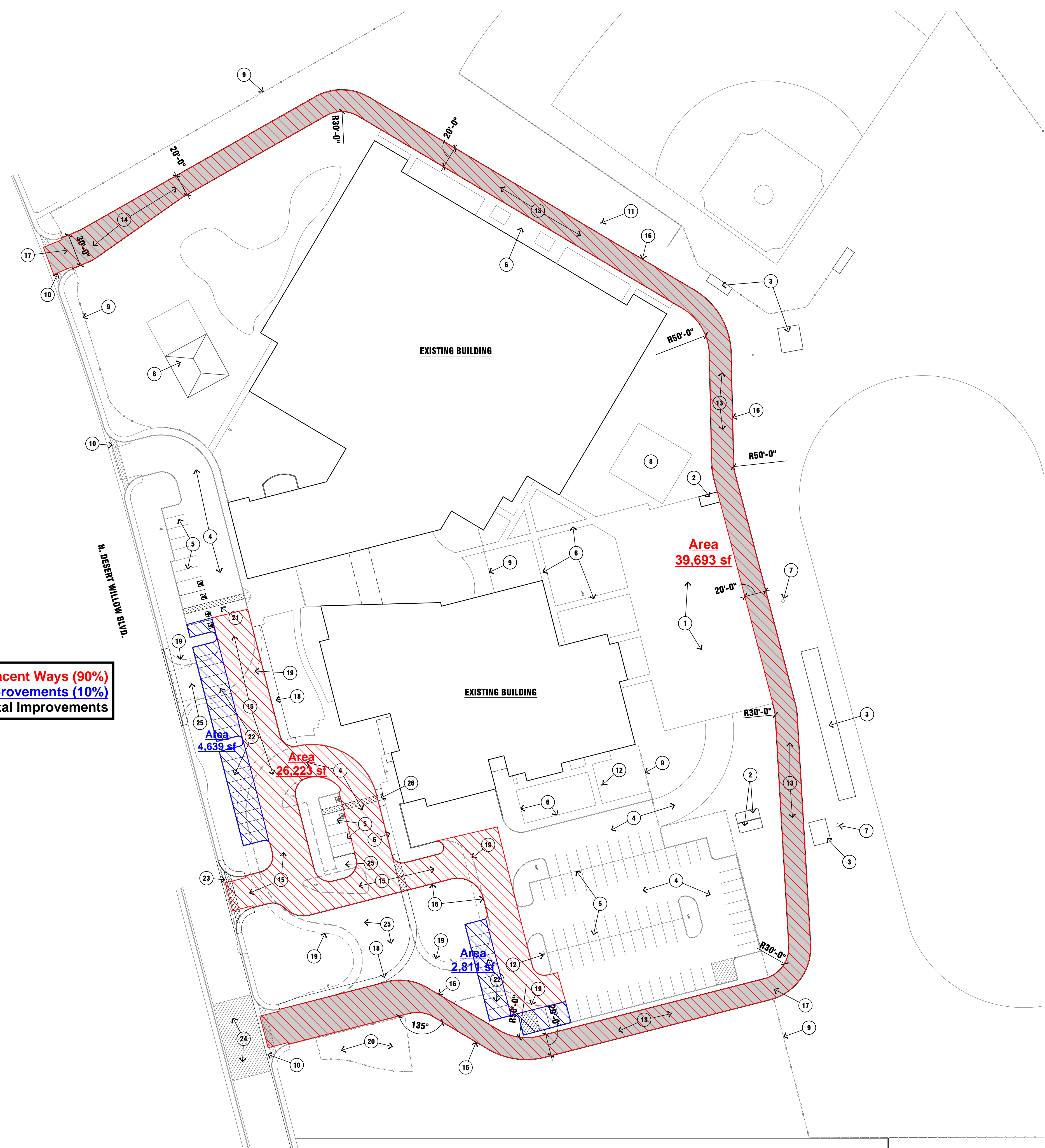
PROPOSED ADJACENT WAYS - ENLARGED SITE PLAN 1" = 50.00'
